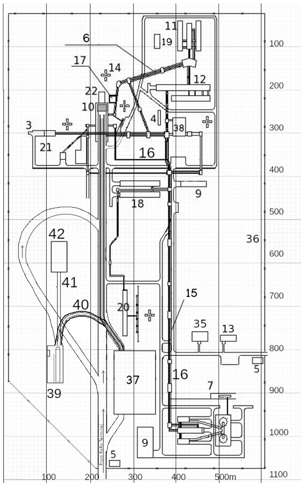
Zenit-Australia Launch Complex
