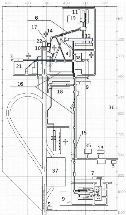
Launch Complex preliminary layout (to scale to the grid). At this picture: 4. Water tower and pump station; 5. Checkpoints; 6. Fuel Pipelines; 7. LOX plant and storage; 9. Power Plant; 10. Launch Pad; 11. Fuel Farm; 13. Fire Fighting Station; 14. Lightning rod towers; 15. Escape Gallery; 16. LOX pipeline; 17. Targeting System; 18. Bottle Facility; 19. Fuel Waste Facility; 21. Oxygen Drain Facility; 22. Flame Duct; 35. Administrative Building; 36. Security Fence; 37. ILV Storage; 38. Command Post.
